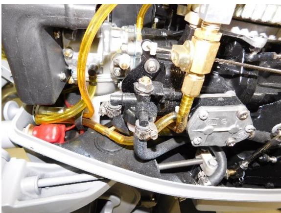
Fig (9) Raider 40HP with Tygon tubing fuel line
