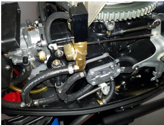
Fig (7) Raider 40HP with USCG compliant lines installed
