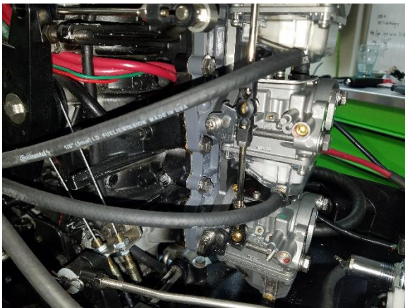
Fig (3) 50HP Carburetor Bowl, installed
