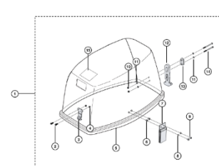
Fig. 24 Top Cowl
