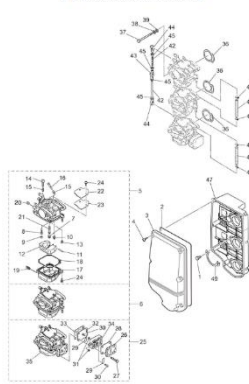
Fig. 4 Intake Silencer • Carburetor
