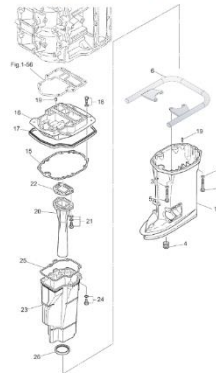
Fig. 13 Drive Shaft Housing
