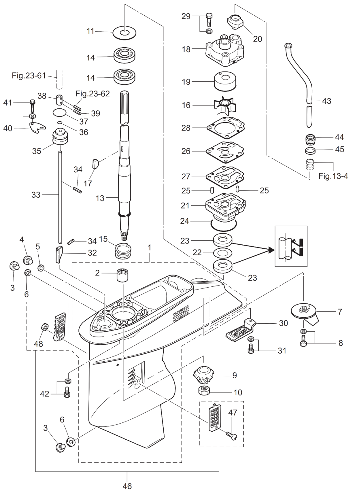
Fig. 14 Gear Case (Drive Shaft)
