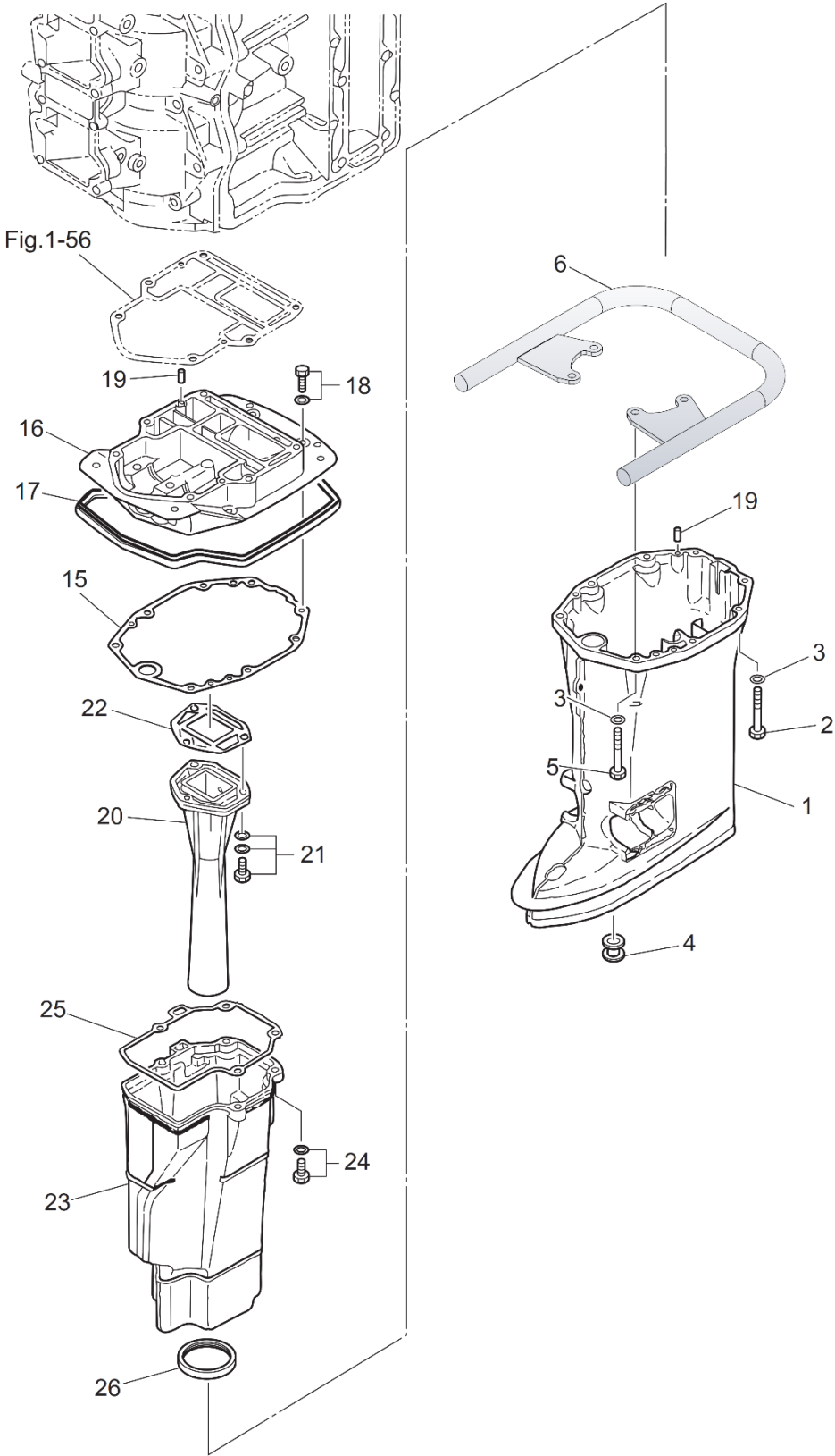
Fig. 13 Drive Shaft Housing
