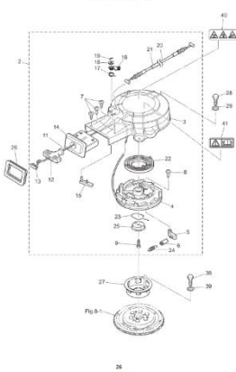
Fig. 7 Recoil Starter
