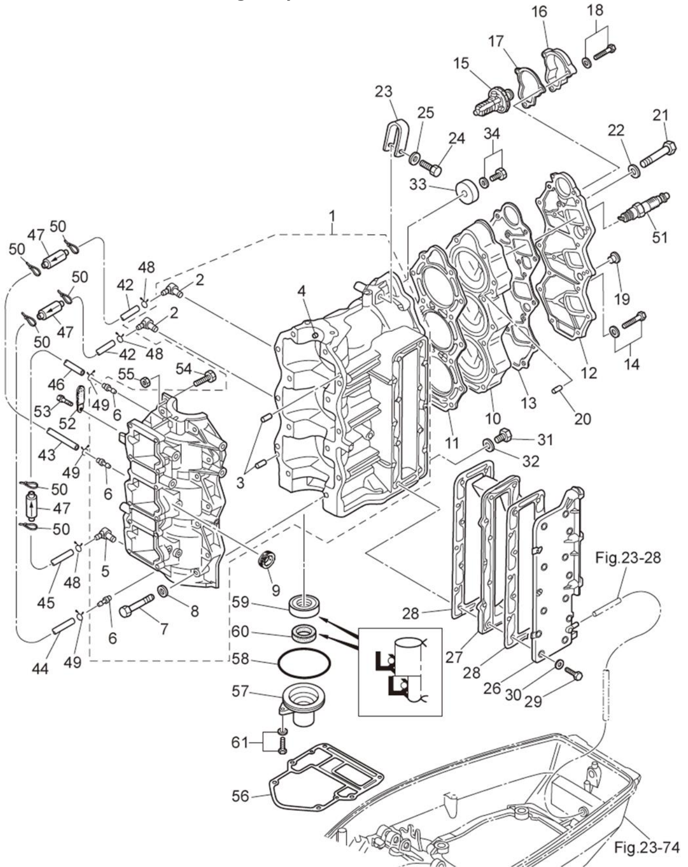
Fig. 1 Cylinder • Crank Case
