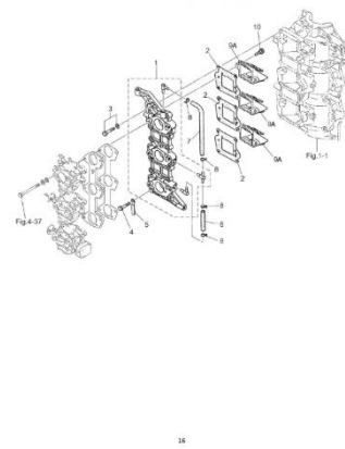
Fig. 3 Intake Manifold • Reed Valve
