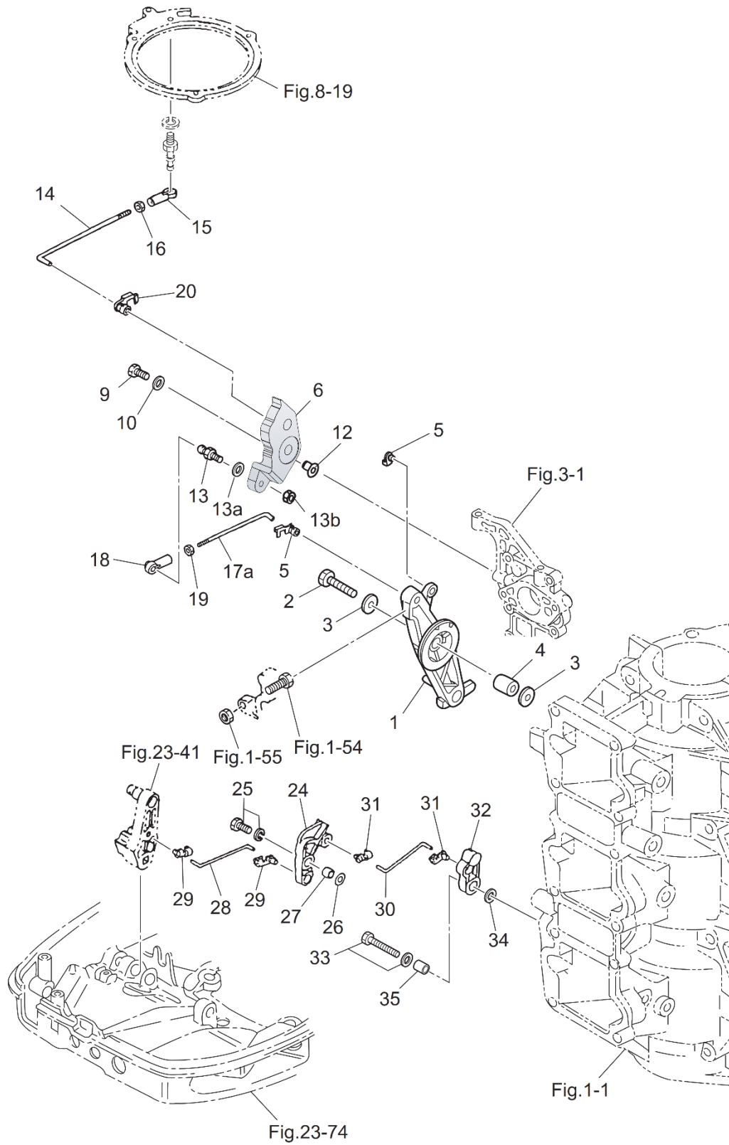
Fig. 6 Throttle
