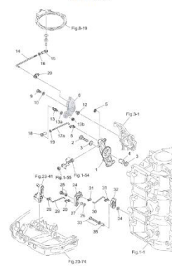
Fig. 6 Throttle
