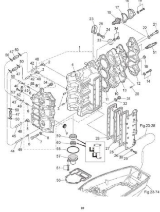
Fig. 1 Cylinder • Crank Case
