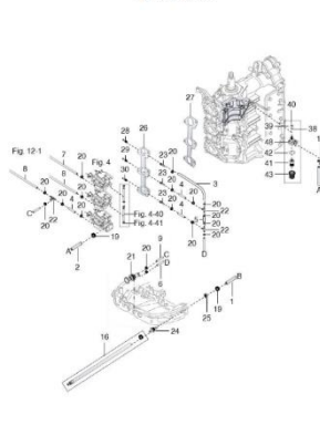
Fig. 5 Fuel System
