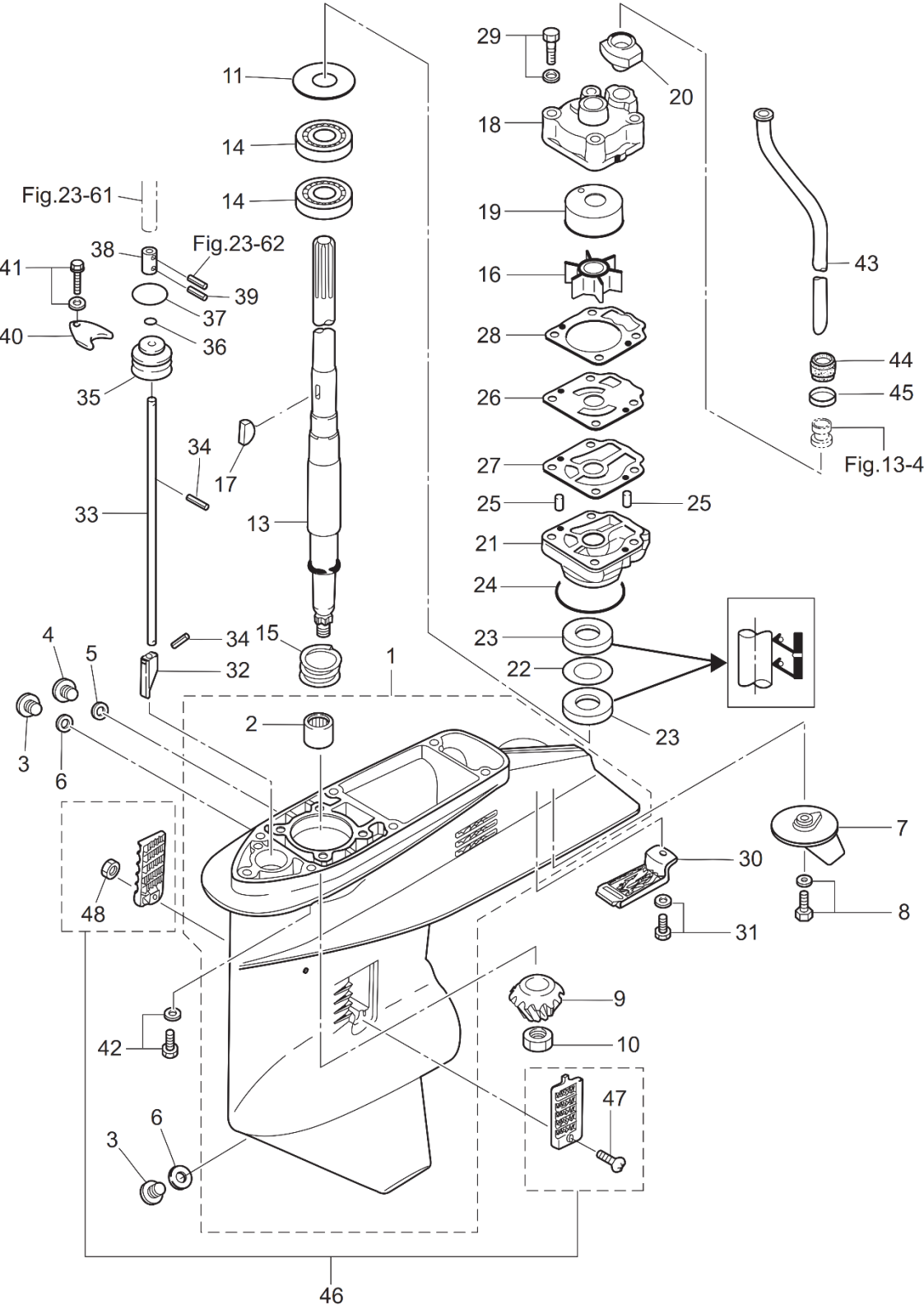
Fig 14. Gear Case (Drive Shaft)
