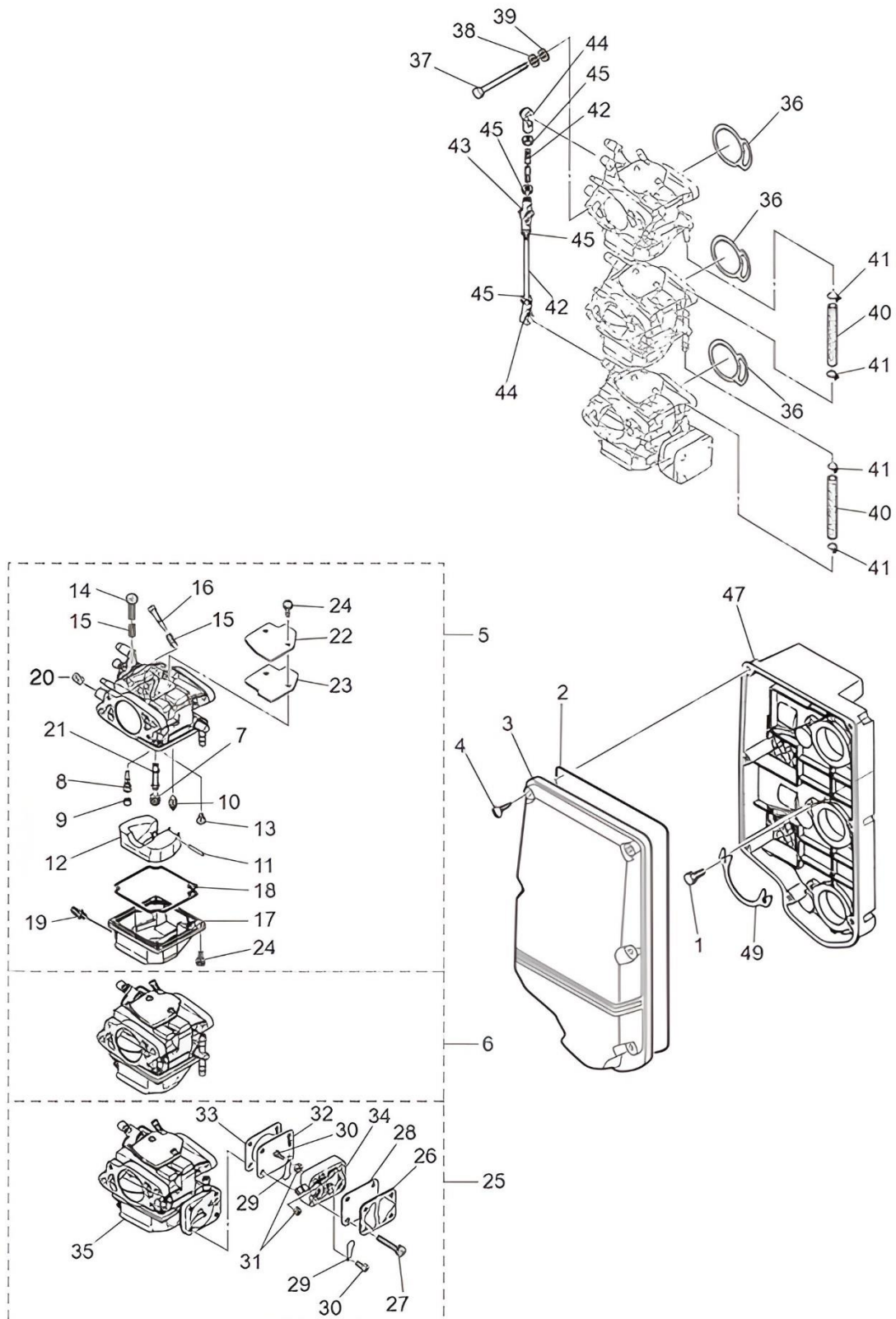
Fig. 4 Intake Silencer • Carburetor
