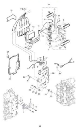
Fig. 10 Electric Parts (C.D. Unit)
