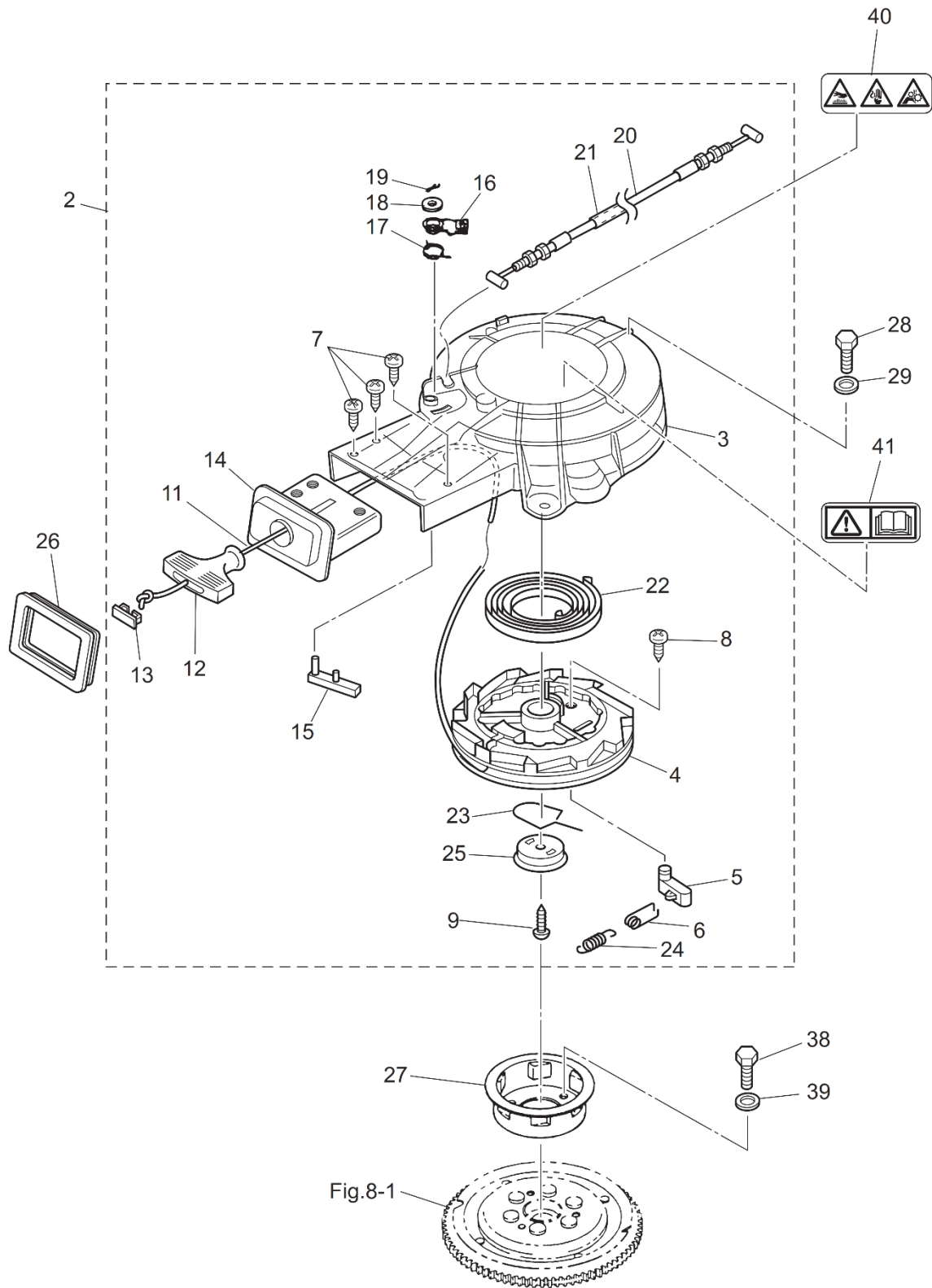
Fig. 7 Recoil Starter
