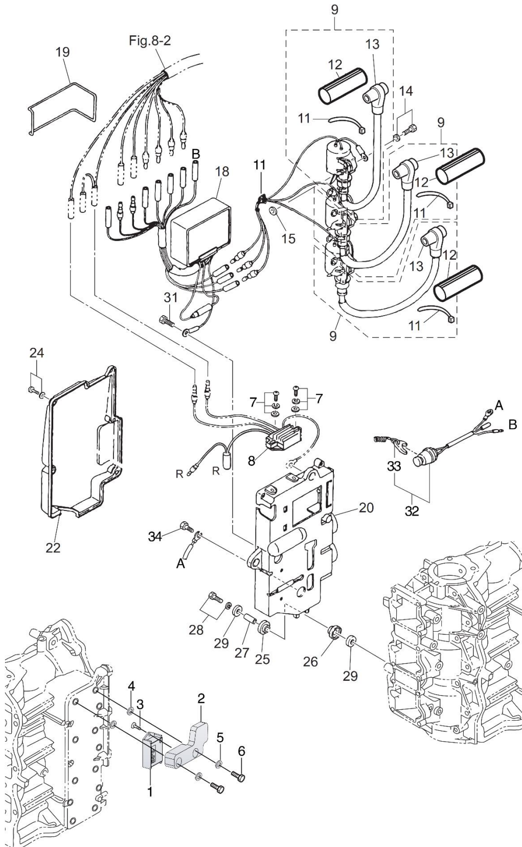
Fig. 10 Electric Parts (C.D. Unit)
