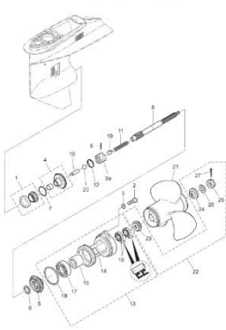
Fig. 15 Gear Case (Propeller Shaft)
