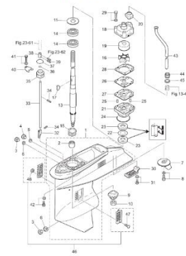
Fig. 14 Gear Case (Drive Shaft)
