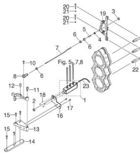
Fig. 12 Dewatering System
